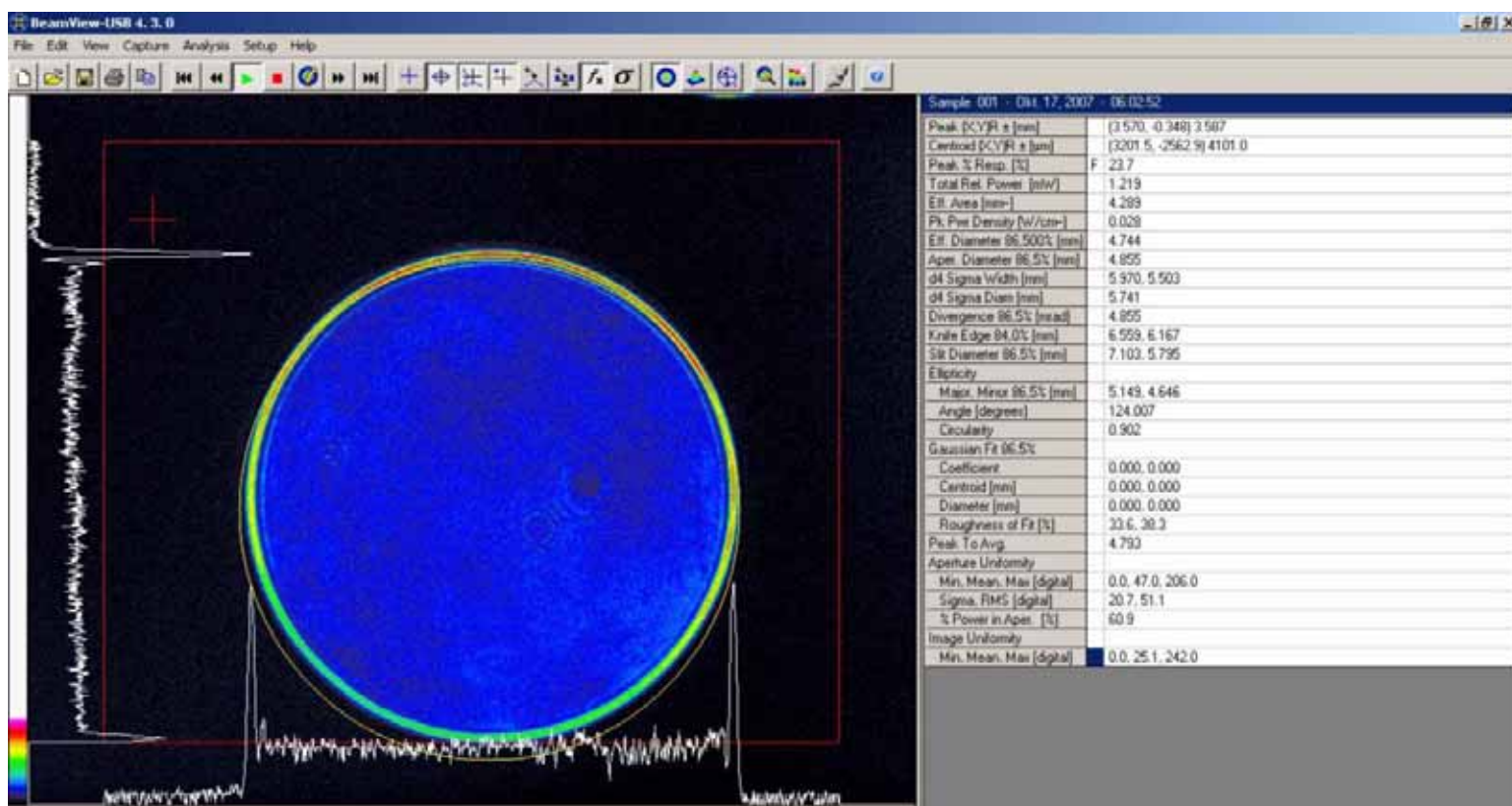
Beam Profile after the \pi Shaper 6_6_VIS
