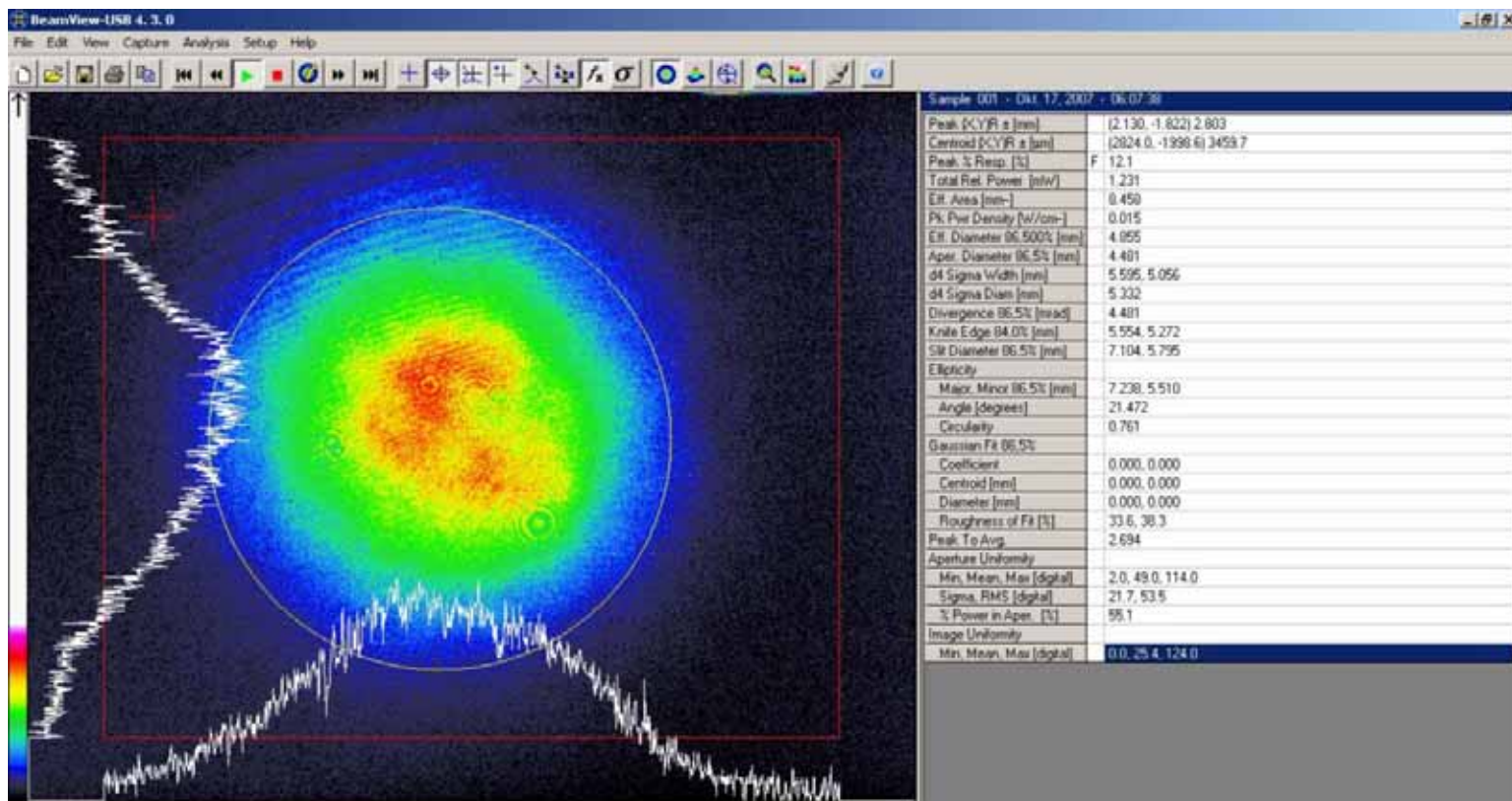
Source Beam Profile, \lambda = 532 nm
