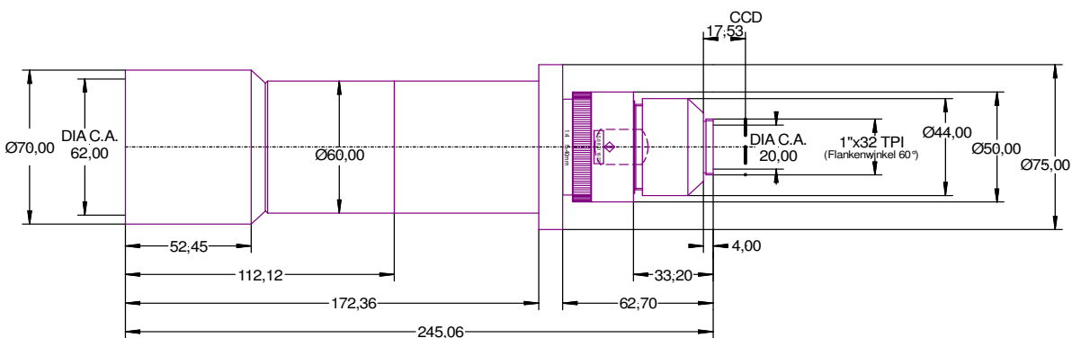
Figure 2: outline drawing
