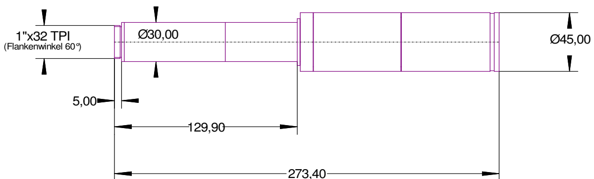
Figure 2: outline drawing
