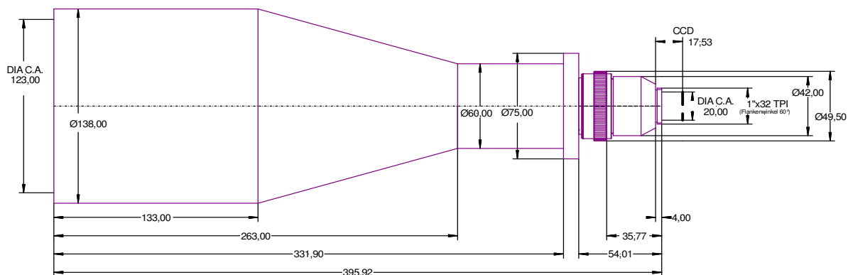
Figure 2: outline drawing
