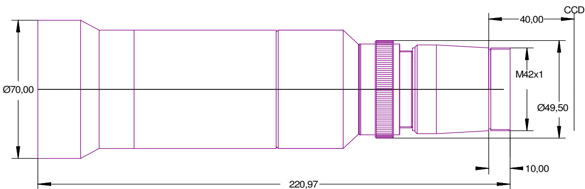
Figure 2: outline drawing
