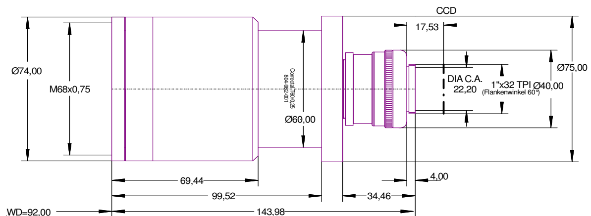
Figure 2: outline drawing
