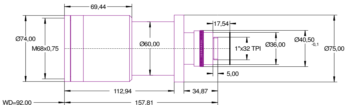
Figure 2: outline drawing
