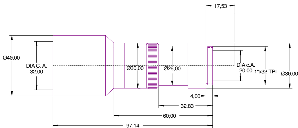
Figure 2: outline drawing
