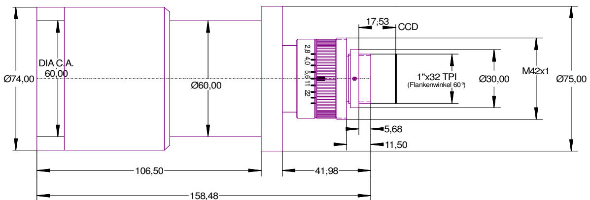
Figure 2: outline drawing
