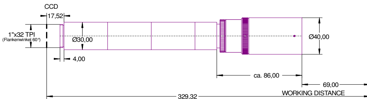
Figure 2: outline drawing
