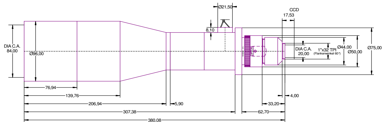
Figure 2: outline drawing
